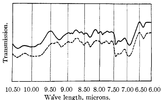
Fig. 6.—Infrared transmission curves of neovitamin A, ---, and vitamin A, —. The percentage transmission is not given as the ordinate because this axis was shifted to permit comparison of the curves. These were, however, plotted from percentage transmission data.
